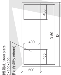
中间支撑详图(俯视图) MID Support Detail
